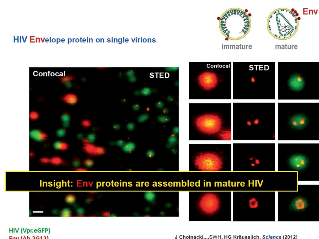
Figure 9. STED nanoscopy of the HIV envelope protein Env on single virions. Confocal microscopy is not able to reveal the nanoscale spatial distribution of the Env proteins; the images of the Env proteins on the virus particles look like 250–350 nm sized blurred spots (orange, left column). STED microscopy reveals that the Env proteins form spatial patterns (center column, orange), with mature particles having their Env strongly concentrated in space (panel in top row of center column, orange).
