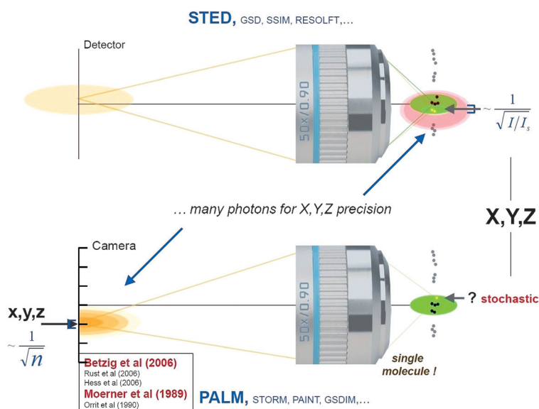
Figure 19. Both in coordinate-targeted and in coordinate-stochastic nanoscopy methods, many photons are required to define or establish, respectively, molecular coordinates at subdiffraction scales. In the coordinate-targeted mode (STED, RESOLFT, etc.), the coordinates of (e.g.) the “on” state are established by illuminating the sample with a pattern of light featuring an intensity zero; the location of the zero and the pattern intensity define the coordinates with subdiffraction precision. In the coordinate-stochastic mode (PALM, STORM, etc.), the coordinates of the randomly emerging “on”-state molecules are established by analyzing the light patterns emitted by the molecules (localization). Precision of the spatial coordinate increases in both cases with the number of photons in the patterns, that is, by the intensity of the pattern. In both families of methods, neighboring molecules are discerned by transiently creating different molecular states in the sample.
