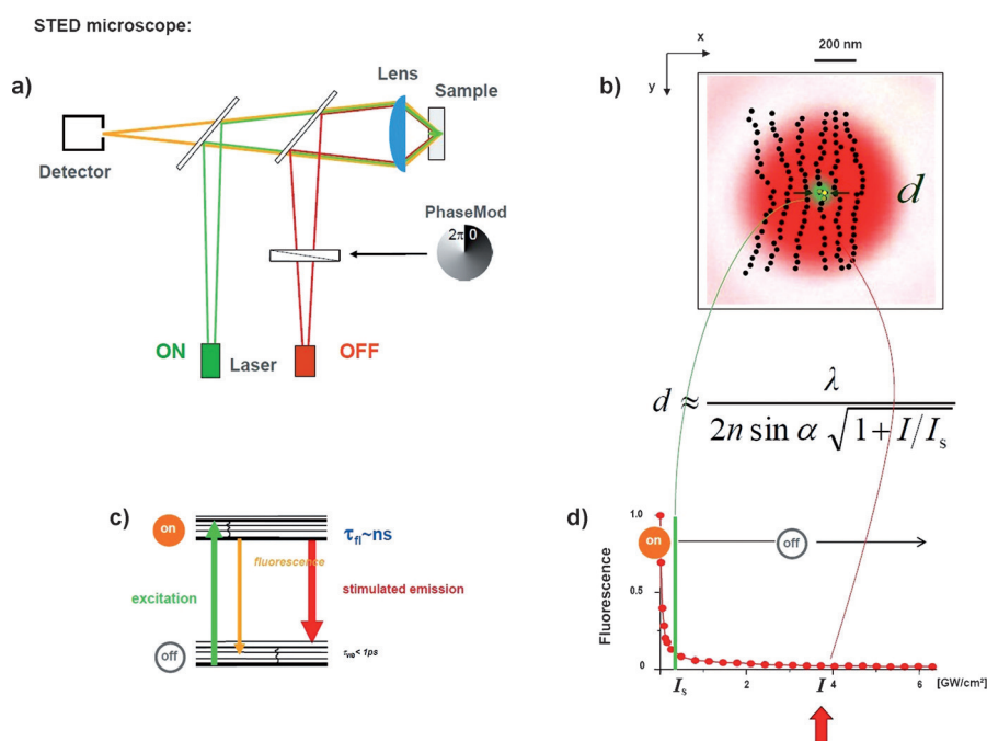
Figure 13. Resolution scaling in the STED/RESOLFT concepts: an extension of Abbe’s equation. The resolution scales inversely with the square root of the ratio between the maximum intensity at the donut crest and the fluorophore-characteristic threshold intensity I_s .
