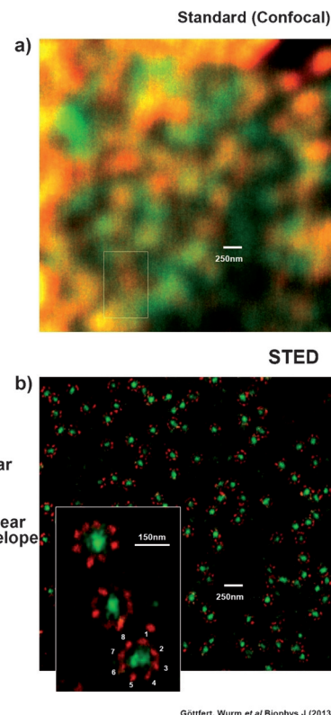
Figure 8. Nuclear pore complex architecture in an intact cell nucleus imaged by a) confocal microscopy (diffraction-limited), and b) STED nanoscopy.
