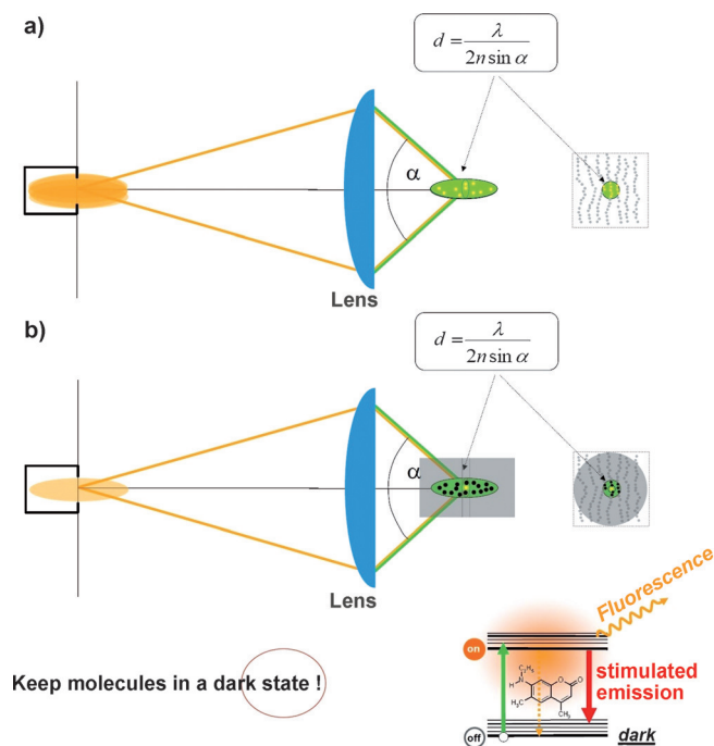
Figure 6. Switching molecules within the diffraction-limited region transiently “off” (i.e. effectively keeping them in a nonsignaling state), enables the separate detection of neighboring molecules residing within the same diffraction region. a) In fluorescence microscopy operating with conventional lenses (e.g. confocal microscopy), all molecules within the region covered by the main diffraction maximum of the excitation light are flooded with excitation light simultaneously and emit fluorescence together. This is because they are simultaneously allowed to assume the fluorescent (signaling) state. b) Keeping most molecules—except the one(s) one aims to register—in a dark state solves the problem. The dark state is a state from which no signal is produced at the detector. Such a transition to the dark “off” state is most simply realized by inducing stimulated emission, which instantaneously forces molecules to their dark (“off”) ground state.
