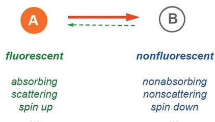
Figure 22. The limiting role of diffraction is overcome by utilizing at least two molecular states to separate features residing closer than the diffraction barrier during the brief period in which the features are jointly illuminated for detection. While fluorescent molecules have been the first type of molecules which have provided such states, other molecules and states are conceivable that are not necessarily of the fluorescent type. This is why one could imagine breaking the diffraction barrier also in a nonfluorescence far-field optical microscope, provided suitable states and state transitions are identified.
