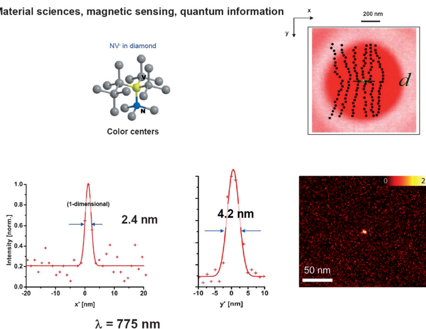
Figure 14. Fluorophores affording virtually unlimited repetitions of the resolution-enabling on-off state transitions provide the present resolution records in far-field optical imaging using STED, in the single-digit nanometer regime. Color centers (charged nitrogen vacancy centers) in diamond hold great potential for various other applications, notably in magnetic sensing and quantum information, which may be eventually read out with diffraction-unlimited spatial resolution using conventional lenses, that is, even when packed very densely at the nanometer scale.
