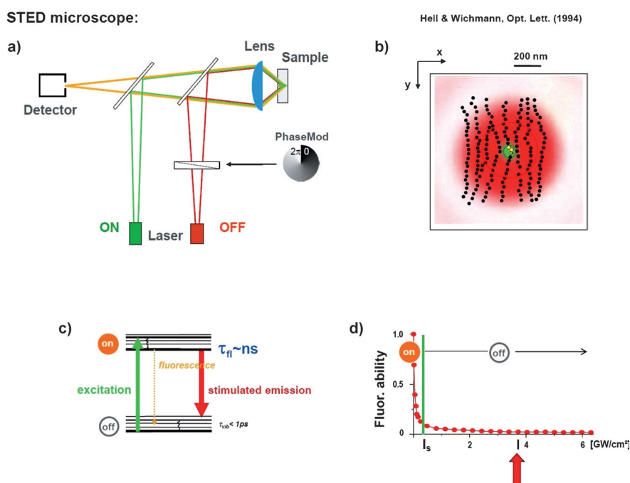
Figure 7. STED microscopy. a) Setup schematic. b) Region where the molecule can occupy the “on” state (green) and where it has to occupy the “off” state (red). c) Molecular transitions. d) For intensities of the STED light (red) equaling or in excess of the threshold intensity I_s , molecules are effectively switched “off”. This is because the STED light will always provide a photon that will stimulate the molecule to instantly assume the ground state, even in the presence of excitation light (green). Thus, the presence of STED light with intensity greater than I_s switches the ability of the molecules to fluoresce off.
