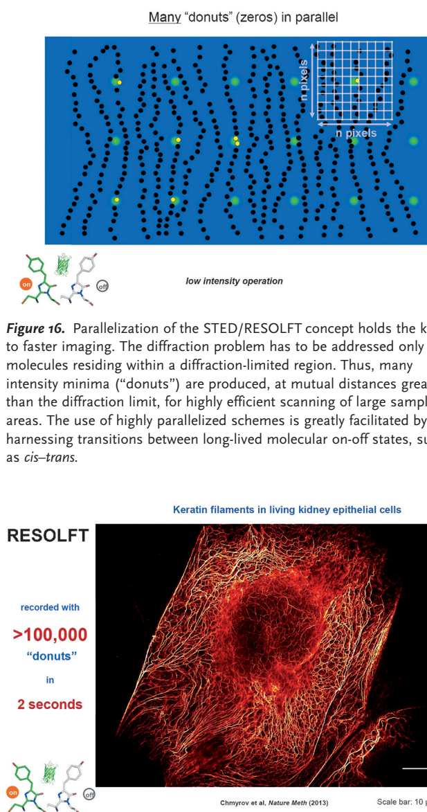
Figure 17. Massively parallelized RESOLFT nanoscopy. Here, an array of ca. 114 000 intensity minima (zeros) was used to image a living cell in two seconds.
