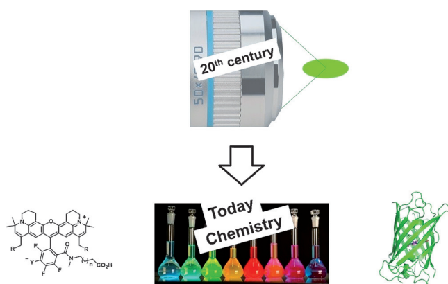
Figure 21. From lenses to molecular switches. Whereas in the 20th century, the focusing quality of the lenses (i.e. excellent aberration correction) was decisive for gaining the best spatial resolution, now it is the molecules and their state transitions which become central to achieving the best resolution. Optimizing molecules towards providing robust and repeatedly executable (on/off) state transitions (STED/RESOLFT) and photon emissions (PALM) is primarily a chemistry problem.
