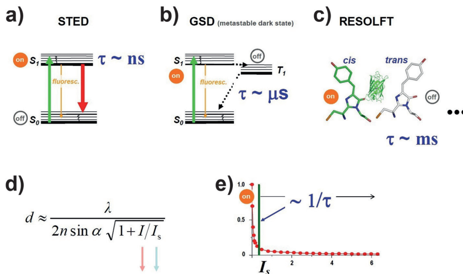
Figure 15. States and state transitions utilized in a) STED, b) GSD, and c) RESOLFT nanoscopy. d) The modified expression for the resolution describes the spatial region in which molecules can still reside in the on state. e) The intensity I_s for guaranteeing the transition from the on to the off state is inversely related to the state lifetime. The longer the lifetime of the involved states, the fewer photons per second are needed to establish the on-off state difference which is required to separate features residing within the diffraction barrier.
