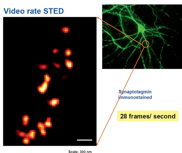
Figure 10. Video-rate STED imaging of synaptic vesicle motion in axon of living hippocampal neurons.
