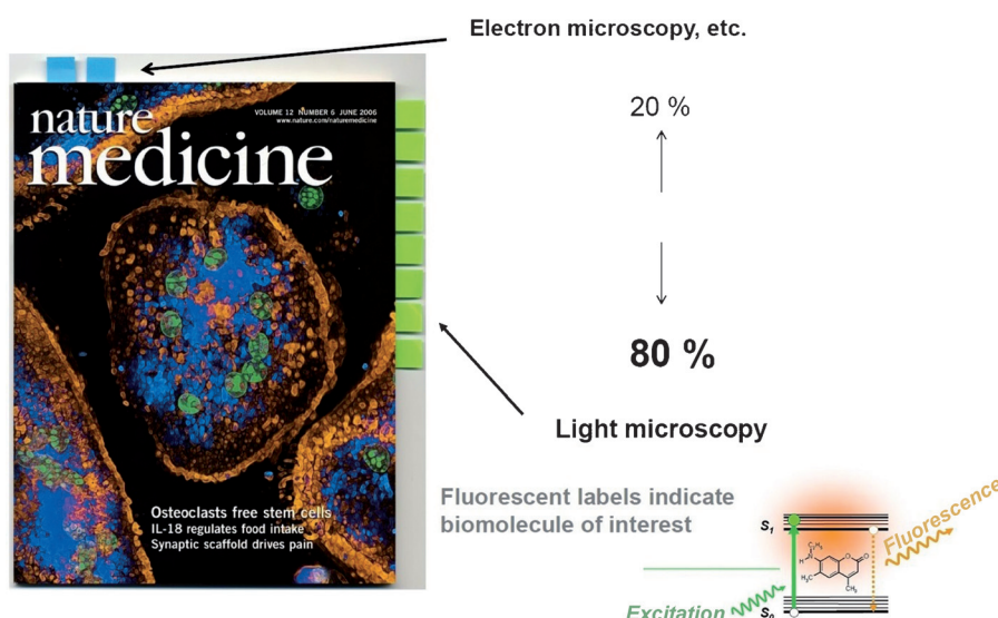
Figure 2. Light microscopy remains the most popular microscopy method in the life sciences, because of a number of distinct advantages such as live-cell imaging and biomolecular specificity. The latter is provided by labeling the biomolecules of interest with fluorescent markers, thus allowing their species-specific detection in the microscope.
