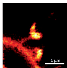
Figure 11. STED nanoscopy in living mouse brain. The recording shows a part of a dendrite of a neuron expressing a yellow fluorescent protein (EYFP) in the cytosol, thus highlighting the neuron amidst surrounding (nonlabeled) brain tissue. The 3–4-fold improved resolution over confocal and multiphoton excitation fluorescence microscopy reveals the dendritic spines (encircled) with superior clarity, particularly the cuplike shape of some of their terminals containing the receiving side of the synapses.
