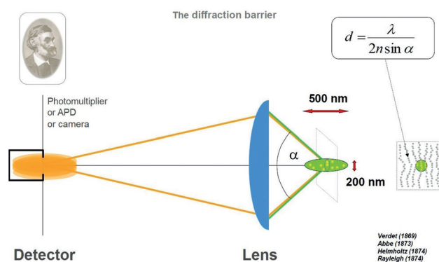
Figure 3. Focusing of light by the microscope (objective) lens cannot occur more tightly than the diffraction (Abbe's) limit. As a result, all molecules within this diffraction-limited region are illuminated together, emit virtually together, and cannot be told apart.
