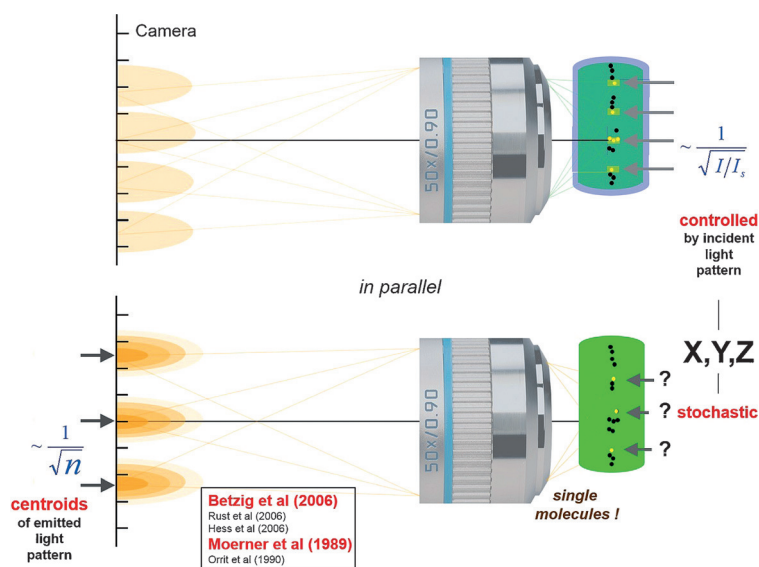
Figure 20. To parallelize STED/RESOLFT scanning, a “wide-field” arrangement with an array of intensity minima (e.g. an array of donuts) may be used. The numbers of molecules at these readout target coordinates do not matter, while PALM requires that there may be only a single “on”-state molecule within a diffraction zone, that is, within the distance dictated by the diffraction barrier. (More precisely: the number of molecules per diffraction zone has to be so low that each molecule is recognized individually.) The position of each on-state molecule is, however, completely random in space. I_s can be regarded as the number of photons that one needs to ensure that there is at least one photon interacting with the molecule, pushing it from one state to the other in order to create the required difference in molecular states. I/I_s is, so to speak, the number of photons which really elicit the (on/off) state transition at the molecule, while most of the others just “pass by”. Similarly, in the PALM concept, the number of photons n in 1/\sqrt{n} is the number of those photons that are really detected at the coordinate-giving pixilated detector (camera), that is, that really contribute to revealing the position of the emitting molecule. In other words, in both concepts, to attain a high coordinate precision, one needs many photons that act.
